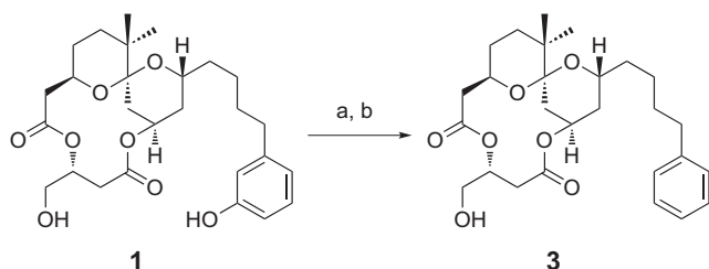
Scheme 1. Synthesis of 3 . Reagents and conditions: (a) N -phenyl triflimide, Et 3 N, CH 2 Cl 2 (91%); (b) Pd(OAc) 2 , Ph 3 P, Et 3 N, HCO 2 H, DMF (25%).
