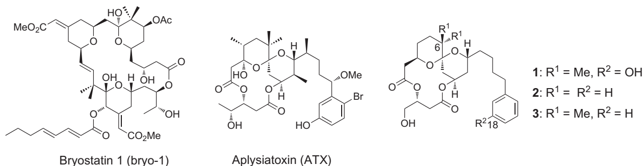
Figure 1. Structure of bryostatin 1 (bryo-1), alysiatoxin (ATX), and the simplified analogues of ATX (1–3).
