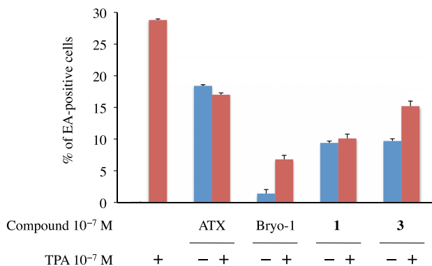
Figure 2. EBV-EA-inducing ability of TPA, ATX, bryo-1, 1 , and 3 . Percentages of EA-positive cells are shown. Sodium n -butyrate (4 mM) was added to all samples to enhance the sensitivity of Raji cells. Only 0.1% EA-induction was demonstrated at 4 mM. The final concentration of dimethyl sulfoxide (DMSO) was 0.4%. Cell viability exceeded 60% in each experiment except for ATX (50%). Error bars represent standard errors of the mean ( n = 3 ).
